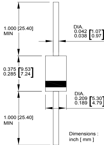
DO-201
